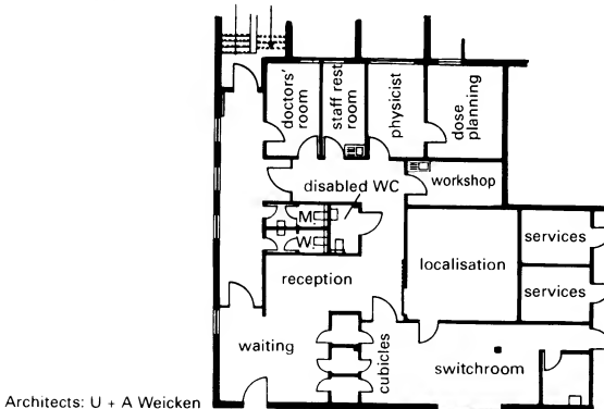
3 Department for linear accelerator
